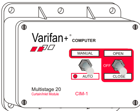
CIM-1 Curtain, Air Inlet and 2 Speed Motors Module (2 mAmp-4 Amp) 1 hp @ 220v
