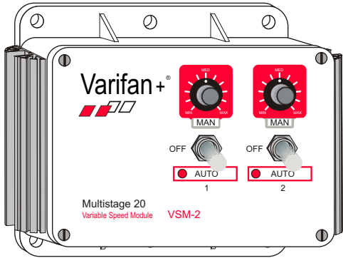
VSM-2 Variable Speed Module (max. 3) 2 variable stages 6 Amp nom. each (0.1 Amp-6 Amp)
