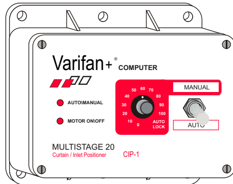
CIP-1 Curtain and Air Inlet Positioner (2 mAmp-3 Amp) 1 hp @ 220v
