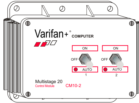
CM10-2 Control Module, 2 single speed stages 10 Amp each (0.1 Amp-10 Amp) 1½ hp @ 220v
