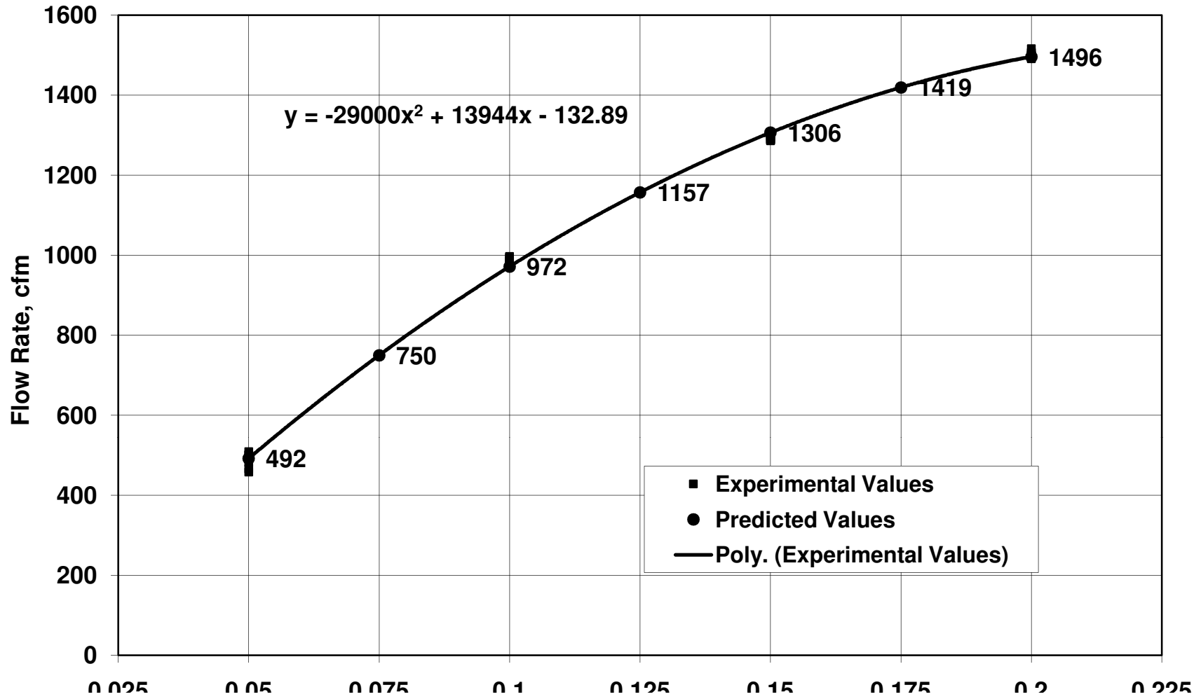
Flow Rate from a BF1200 at a weight placement of 1.5 inches
