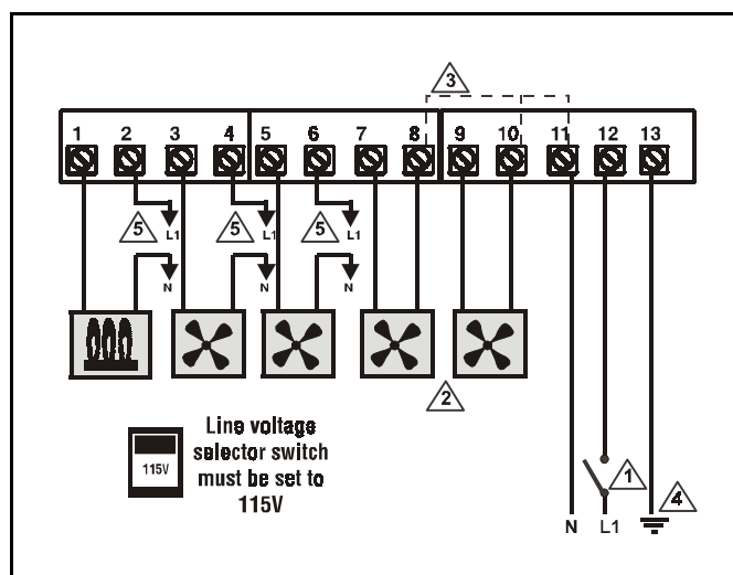
Fig. 1 Four Fans (115V) and One Heating Unit (115V)
