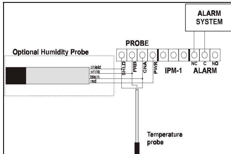
Fig. 4. Probes and Alarm Wiring
