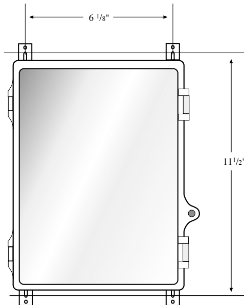
Figure 1: Mounting Dimensions
