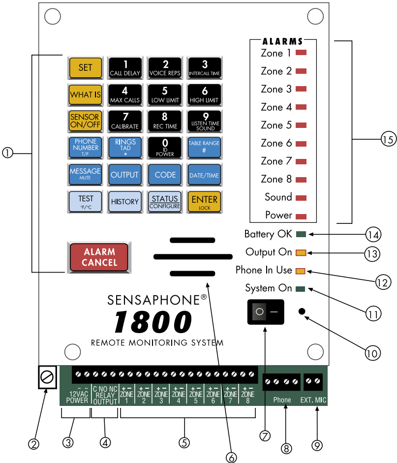
Figure 1: Sensaphone 1800 diagram
