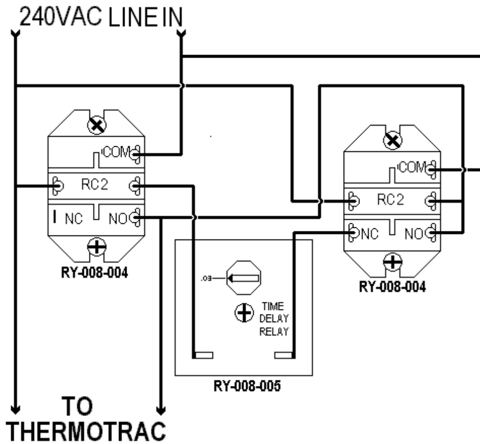
RY-008-003 WIRING DIAGRAM
