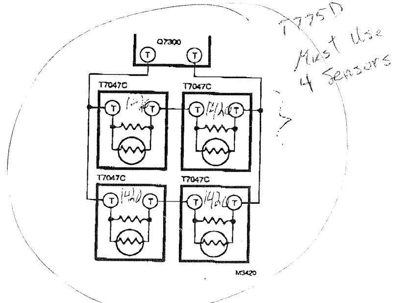
Fig. 7—Four T7047C1025 Sensors providing a temperature averaging network for a T7300/Q7300 Thermostat /Subbase.
