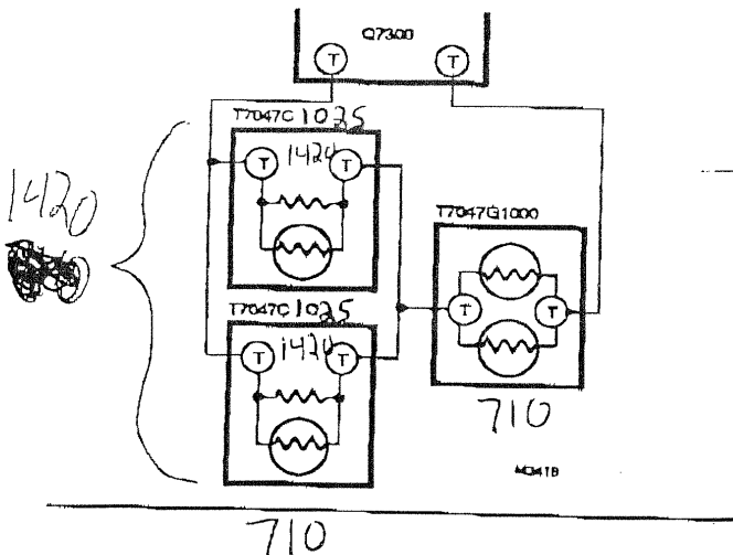
Fig. 6—Two T7047C1025 and one T7047G1000 Sensors providing a temperature averaging network for a T7300/Q7300 Thermostat/Subbase.
