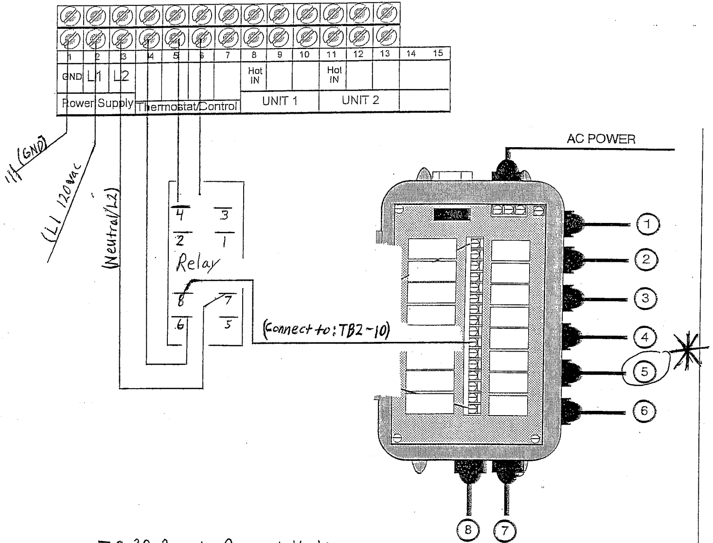
Figure 3. CABLE ROUTING DIAGRAM
