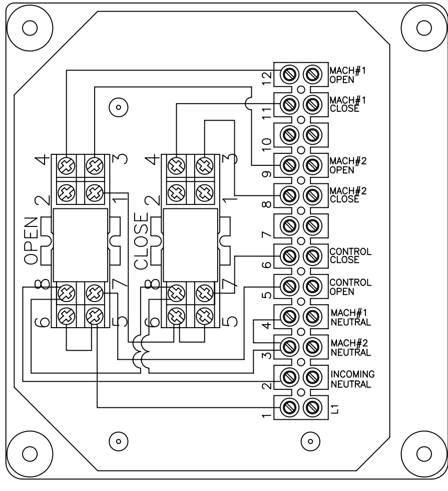
RCIR-1 INTERNAL BOX VIEW
